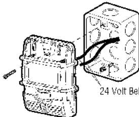
PRE-WIRED INSTALLATION
