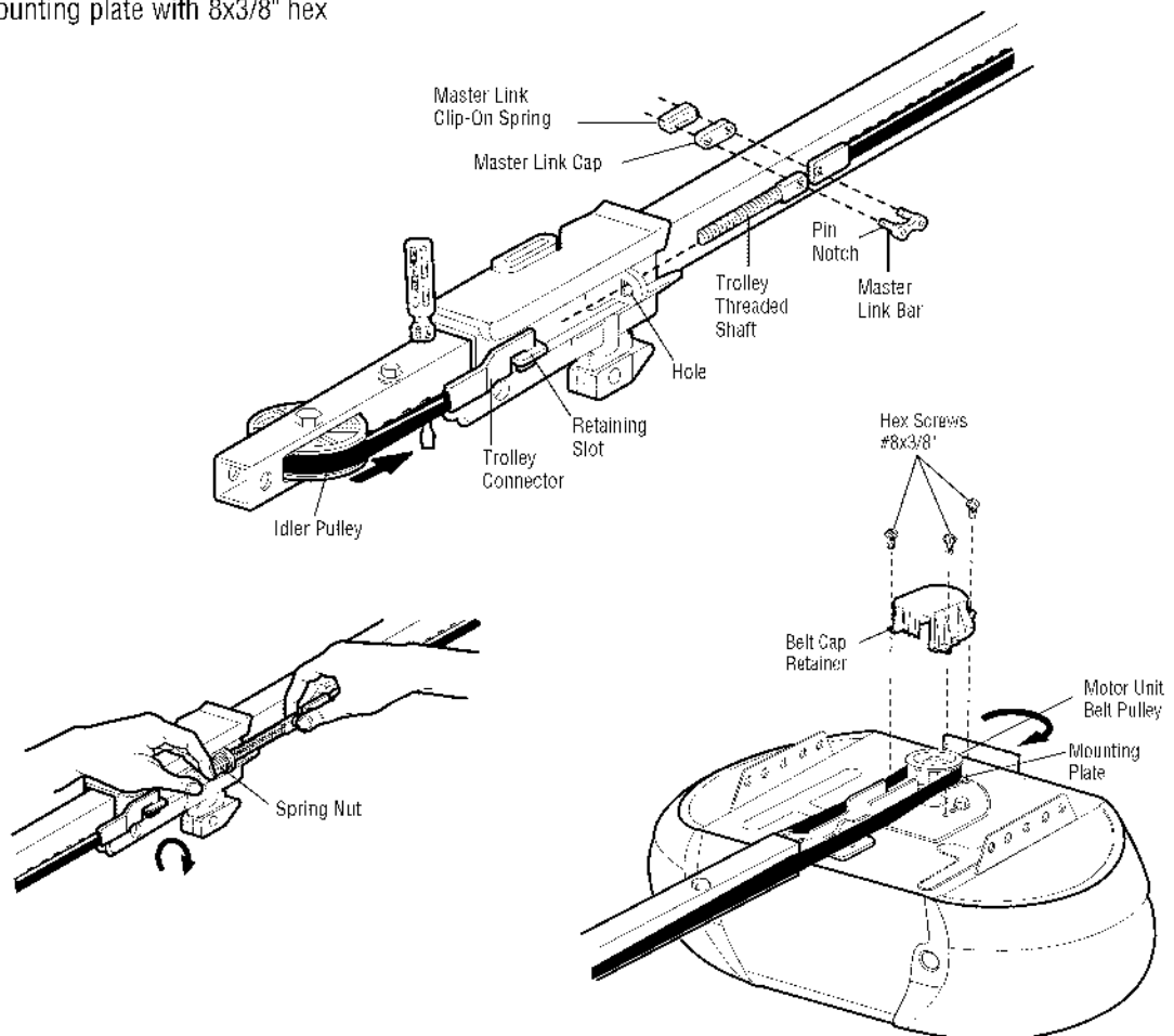
Spring/Trolley Nut
