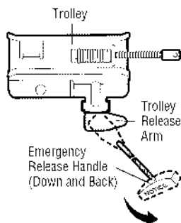
To reconnect
